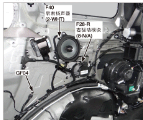
120.行李箱右侧
